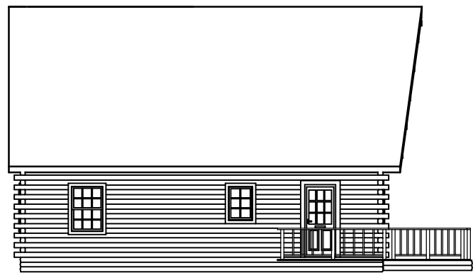
LEFT ELEVATION
